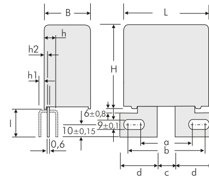
2-Draht Version
