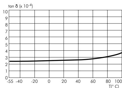
Dissipation factor change versus temperature ( f = 1\text{ kHz} ) (general guide).
