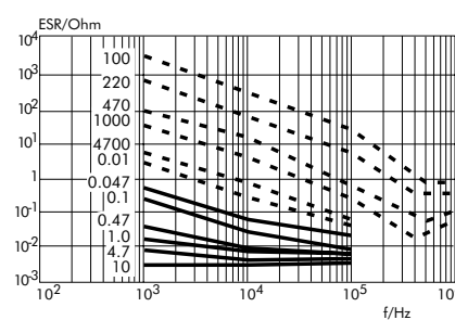
ESR change versus frequency (general guide)
