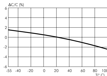
Capacitance change versus temperature ( f = 1\text{ kHz} ) (general guide).
